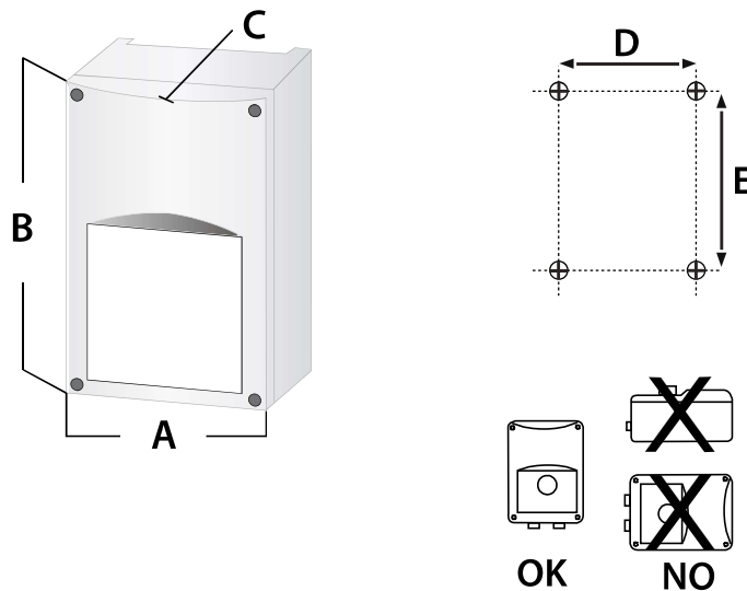
Dimensions (mm)
